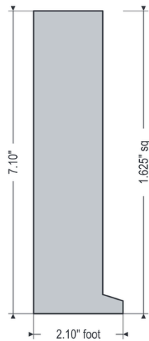
ETBB10 Reach bar, 1.625 sq, end foot
